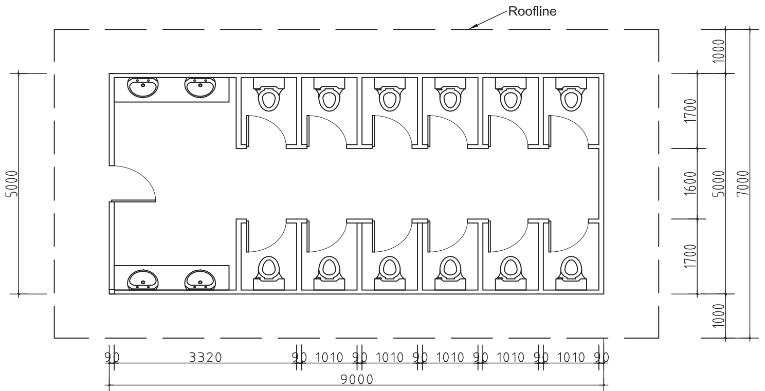
FLOOR PLAN
