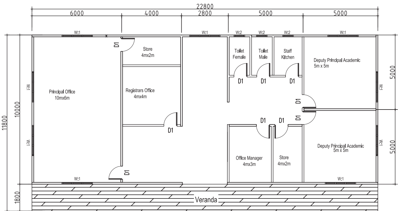
FLOOR PLAN
