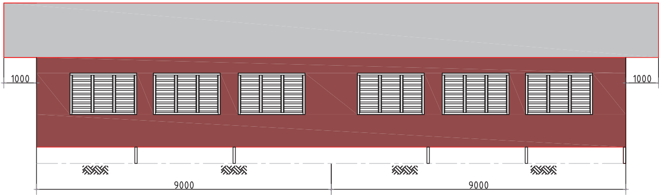
Rear Elevation
