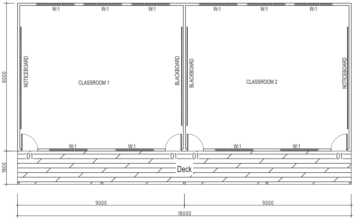
FLOOR PLAN
