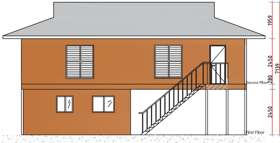
LEFT SIDE ELEVATION SCALE 1:100
