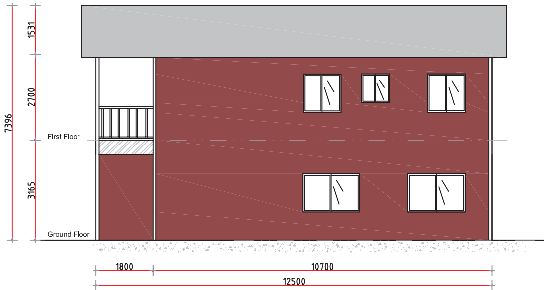
LEFT ELEVATION 1:100
