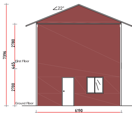
BREA ELEVATION 1:100
