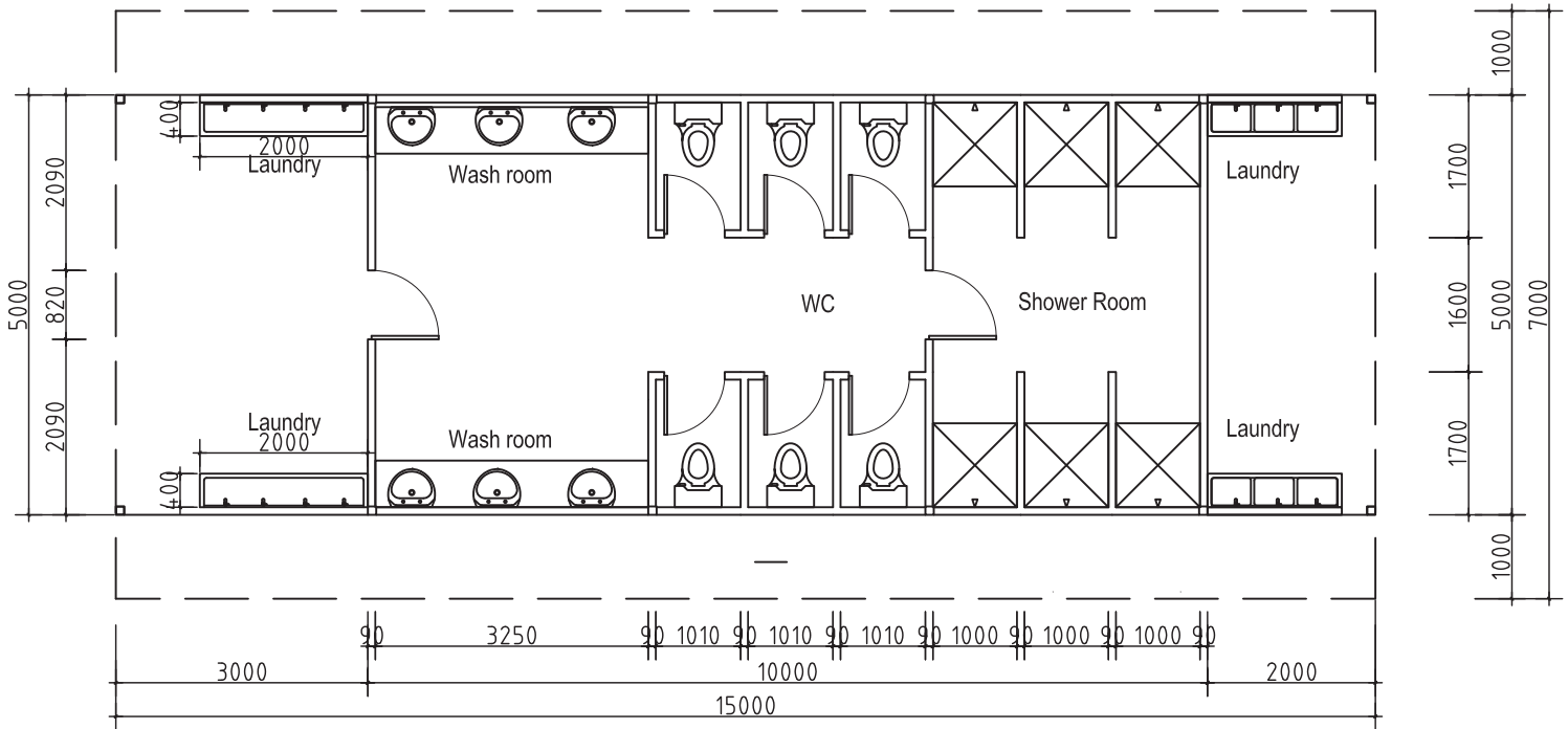
FLOOR PLAN
